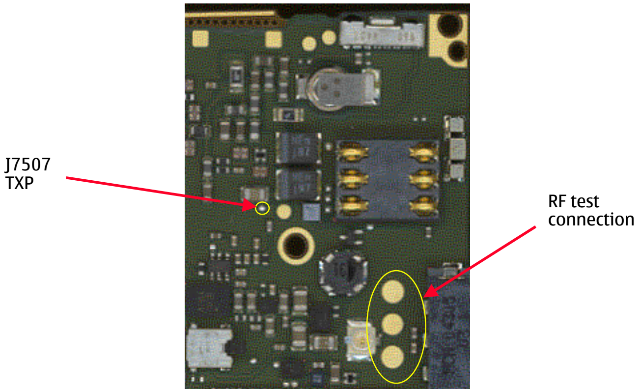
Figure 2: Bottom view
