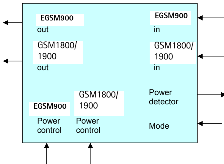
Figure 9: Power amplifier
