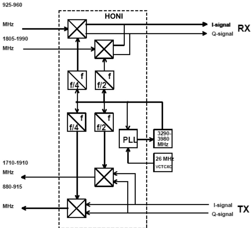
Figure 3: RF frequency plan
