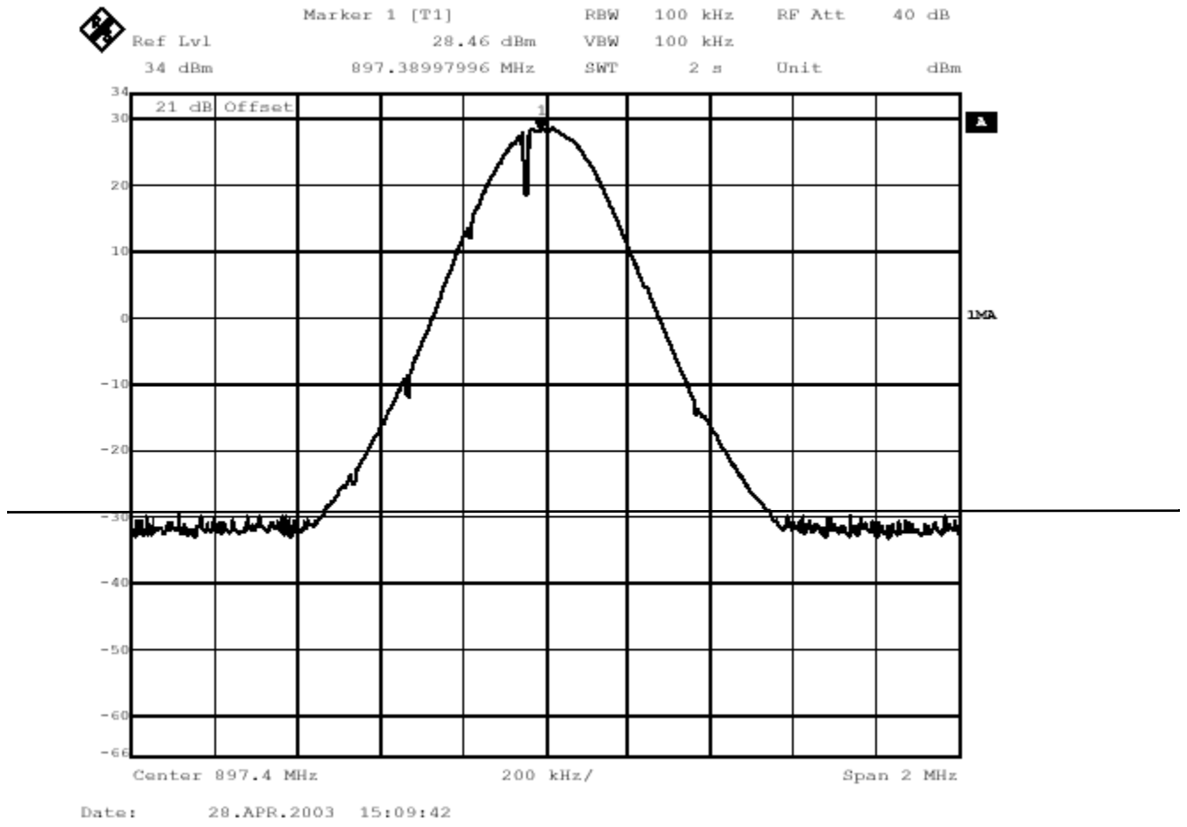
Figure 10: Tx out signal, 900 band burst mode, channel 37
