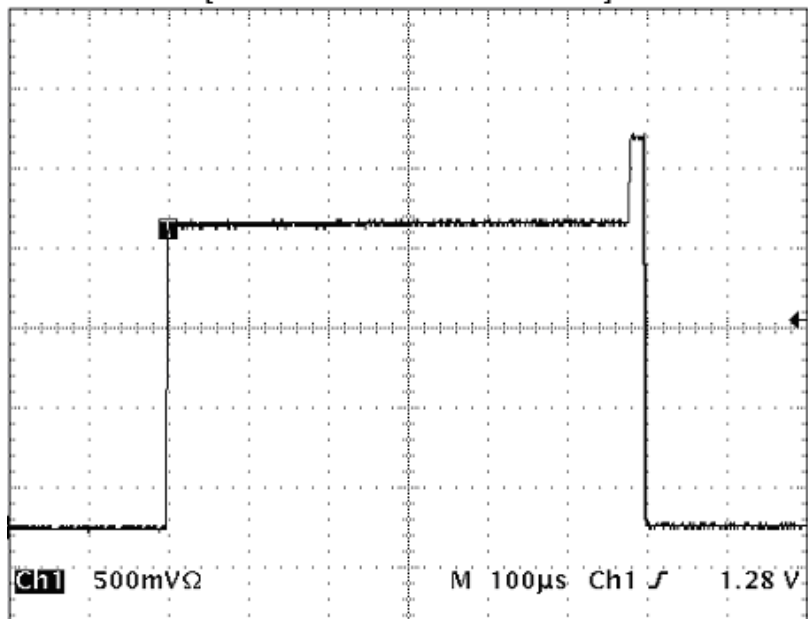
Figure 16: I_ref 900 power level 8 at R7701/C7701
